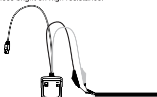
Figure 5 Continuity test
