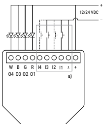
Fig. 1 Wiring in Lights mode
