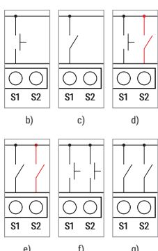
Fig. 3. Cover control profile
