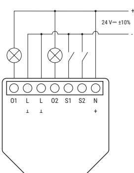
Fig. 2. Dual-channel switch, 24-30 V~ power supply
