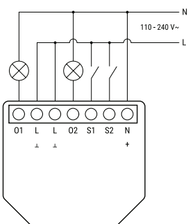
Fig. 1. Dual-channel switch, 110-240 V~ power supply
