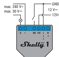
EN Fig. 3. 12 V~ stabilized power supply
