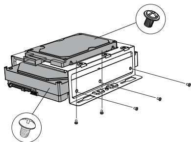
HDD/SSD installation
